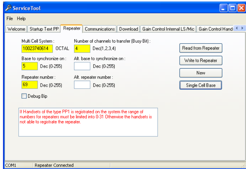
Figure 2-4 Repeater Page of the Service Tool Program
