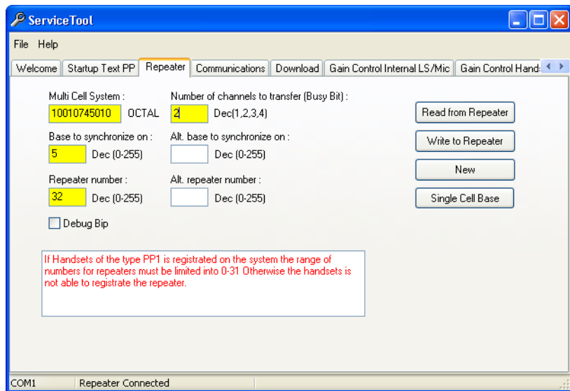
Figure 2-6 Repeater Page of the ServiceTool Program
