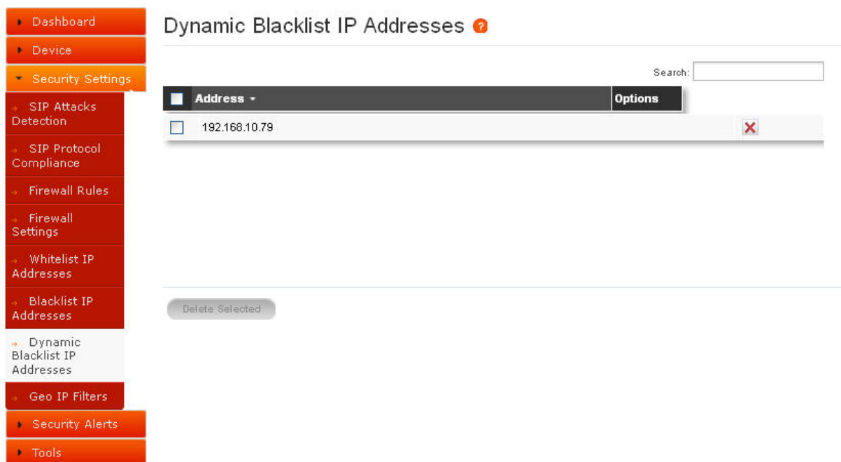
Figure 24: Dynamic Blacklist IP Addresses
