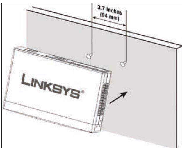
Proper Wall-Mount Orientation (Horizontal)
