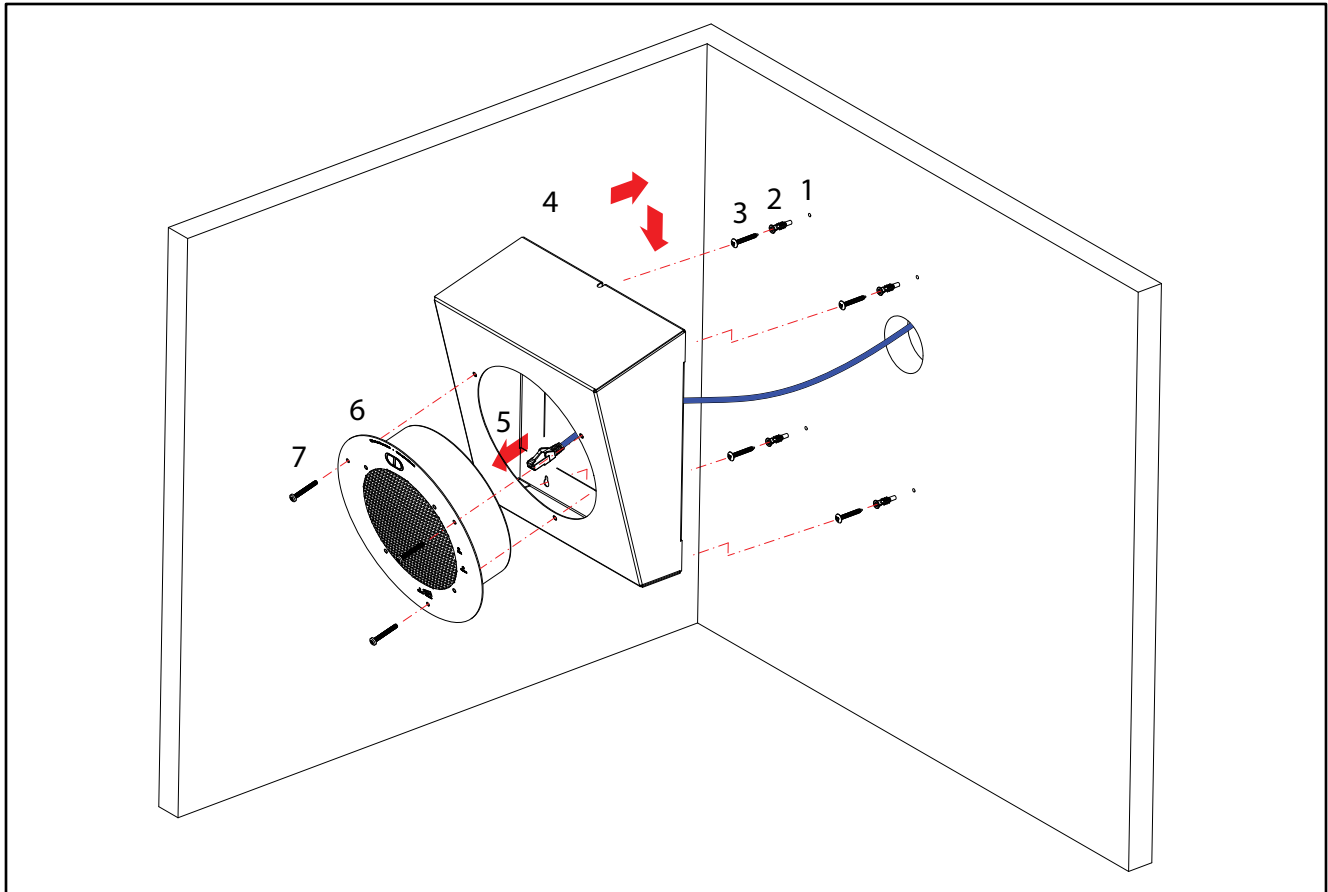
Exploded View
